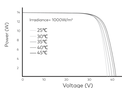
P-V Curve
